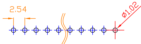
Recommended P.C.Board Hole Layout
