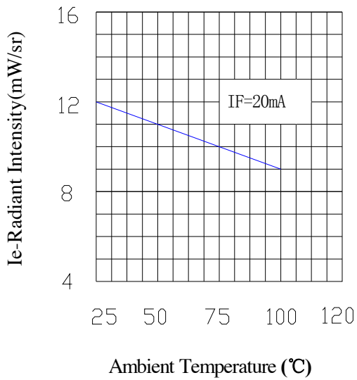
Fig.7 Relative Intensity vs. Ambient Temperature (°C)
