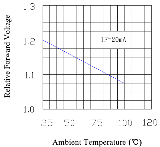
Fig.8 Forward Voltage vs. Ambient Temperature (°C)
