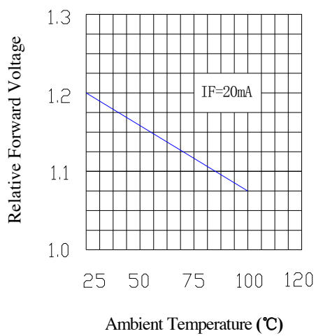
Fig.8 Forward Voltage vs. Ambient Temperature (°C)
