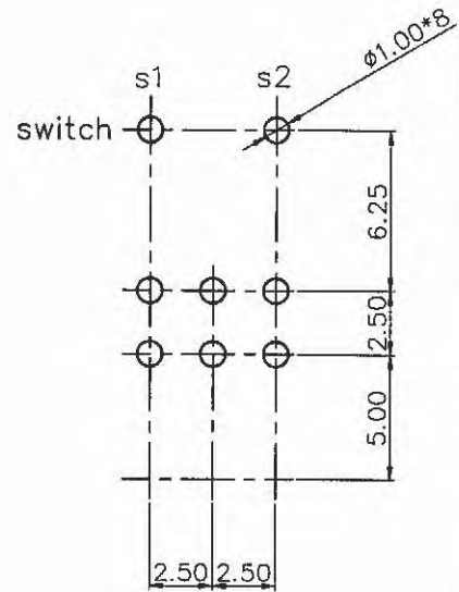
Mounting hole detail
